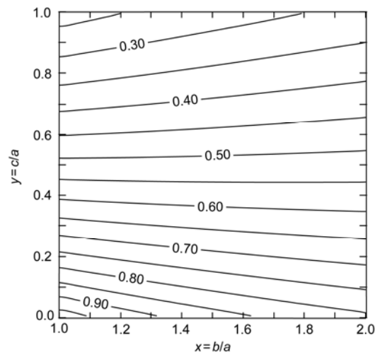
Figure 8 The contours of the earth pressure coefficient at rest K_o .
