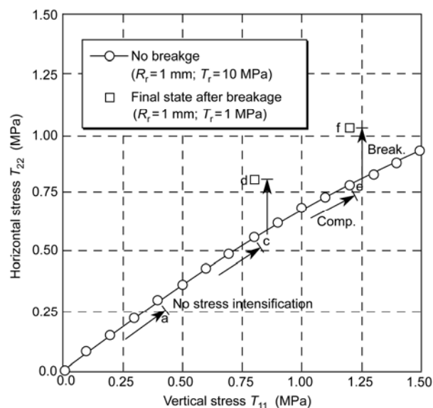
Figure 10 The horizontal stress intensification induced by particle breakage.
