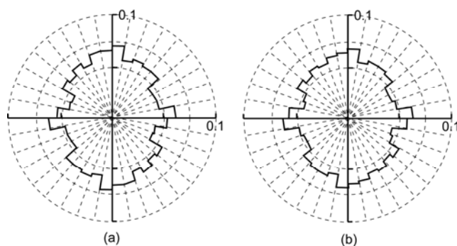
Figure 5 The polar distributions of the contact angle before and after lubrication. (a) At state e; (b) at state f.
